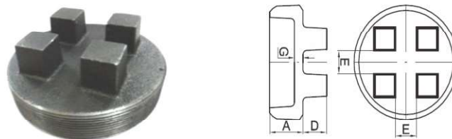
Fig No. 31B - SLOTTED HEAD PLUGS (P SLOTTED)
