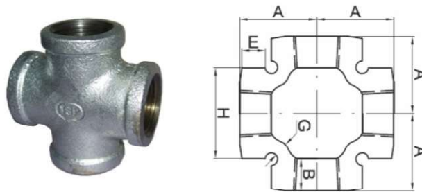
Fig No. 19A - CROSSES (BCR)
