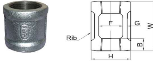
Fig No. 24B - COUPLINGS BANDED (BS)
