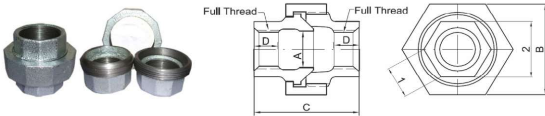
Fig No. 35C - UNION FEMALE CONICAL JOINT IRON TO IRON SEAT (CU)
