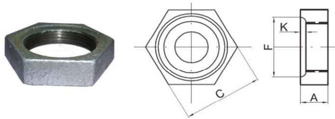
Fig No. 29 - LOCKNUTS (LN)
