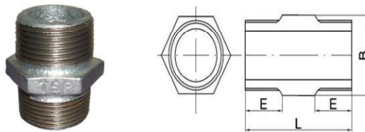
Fig No. 32 - NIPPLES (N)
