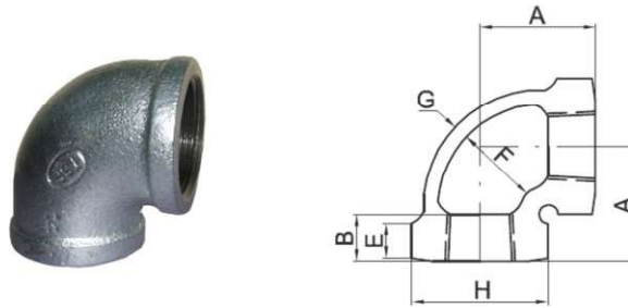
Fig No. 3 - ELBOWS 90° BANDED (BL 90)
