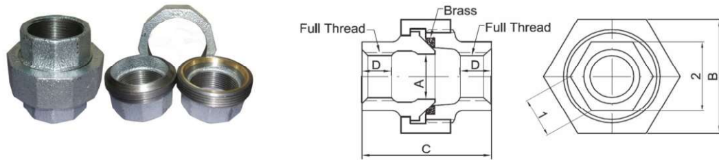
Fig No. 35B - UNIONS FEMALE CONICAL JOINT BRASS TO IRON SEAT (CU BRASS)
