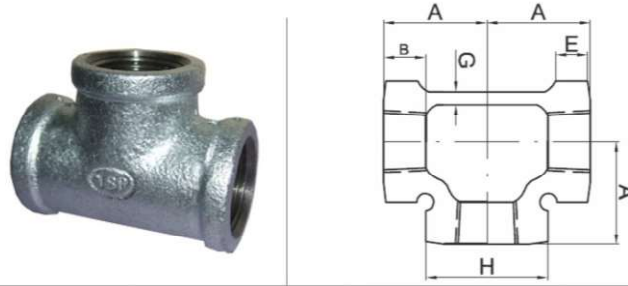
Dimension of Class 150 - (in Inch)
