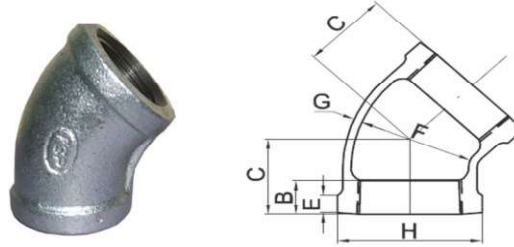
Fig No. 6 - ELBOWS 45° BANDED (BL 45)
