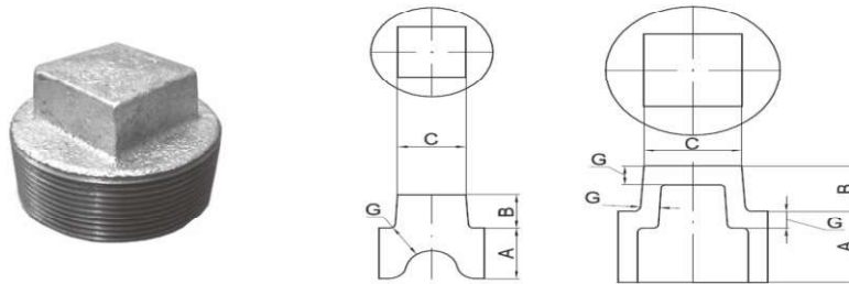
Fig No. 31A - SQUARE HEAD PLUGS (P SQUARE)
