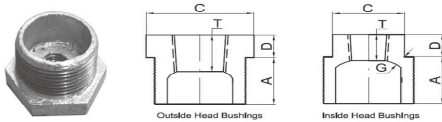
Fig No. 30 - BUSHINGS (HB)
