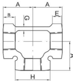
Fig No. 13 - TEES BANDED (BT)
