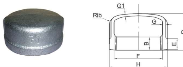
Fig No. 21A - ROUND CAPS BANDED (RC)
