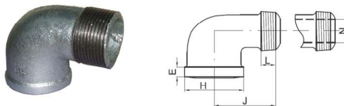
Fig No. 7B - STREET ELBOWS 90° BANDED (BSL 90)
