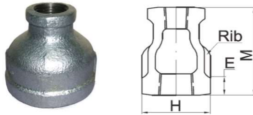
Fig No. 26 - REDUCING COUPLINGS BANDED (BRS)
