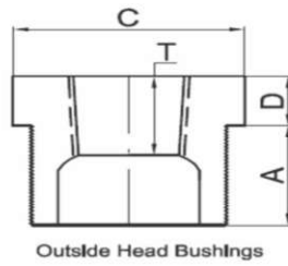
Fig No. 30 - BUSHINGS (HB)
