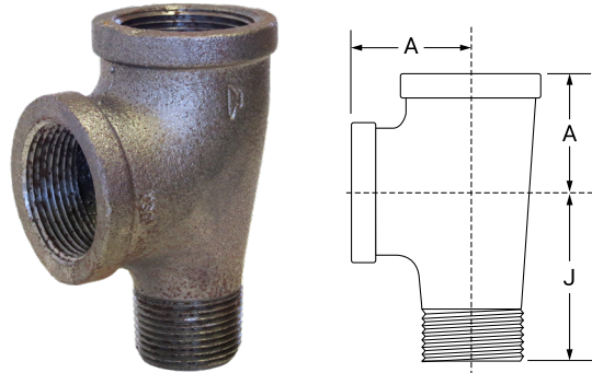
Fig. 1106, 1106R Straight Street or Service Tee (Class 150 Standard) Reducing Street or Service Tee (Class 150 Standard)
